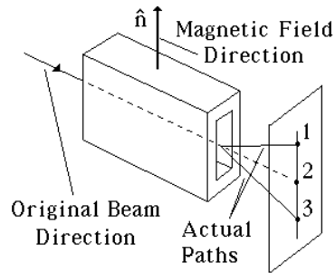
Figure 5.4: Stern-Gerlach Apparatus
