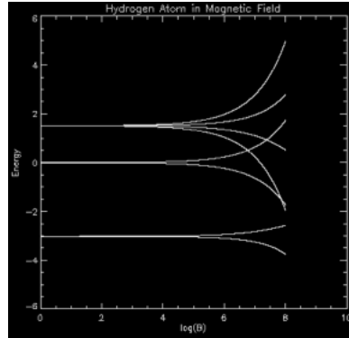
Figure 8.2: Hydrogen Atom In a Magnetic Field - Zeeman Effect
