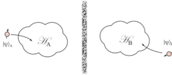
Figure 4.5: Hilbert space for 2 quantum systems independent of one another
