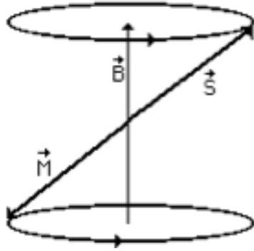
Figure 7.1: Motion of Spin
