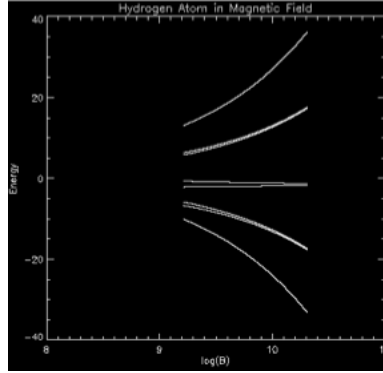
Figure 8.3: Hydrogen Atom In a Magnetic Field - Paschen-Bach Effect
