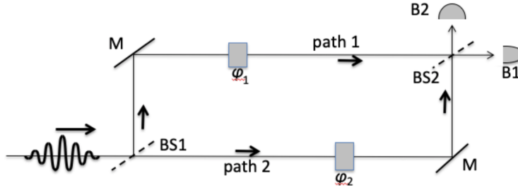
Figure 10.9: Mach-Zehnder interferometer experiment. A photon traverses a beam splitter, travels on two phase-shifted paths to another beam splitter, and is detected.
