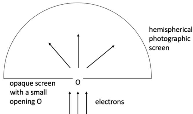
Figure 10.8: Einstein's Thought experiment. Each electron diffracts widely, reaching the entire screen simultaneously, yet only one point shows an impact. How do the other points instantaneously remain dark? Does this violate Special Relativity?
