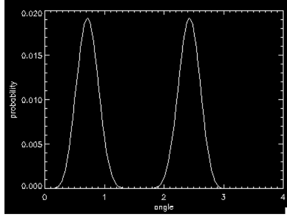
Figure 5.3: Most Likely Angles
