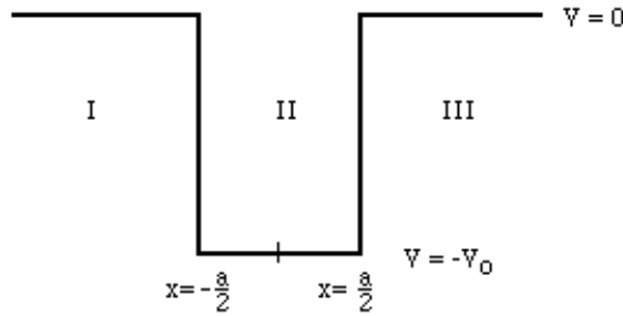
Figure 6.7: Finite Square Well
