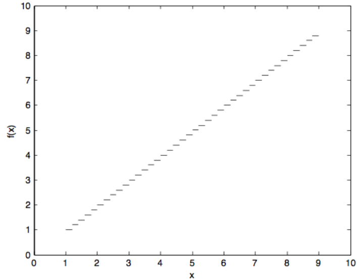
Figure 2.1: Staircase Function
