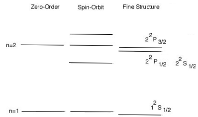
Figure 8.5: Fine Structure Energy Levels
