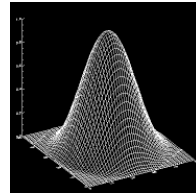
Figure 7.8: |\psi_{01}|^2
