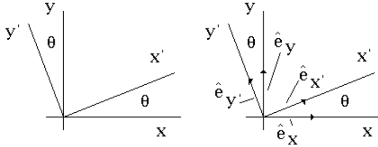
Figure 5.1: Rotation of Axes
