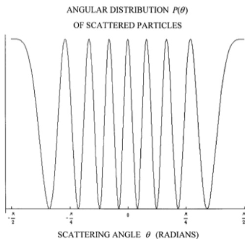
Figure 6.21: Angular Distribution of scattered particles from double narrow slits
