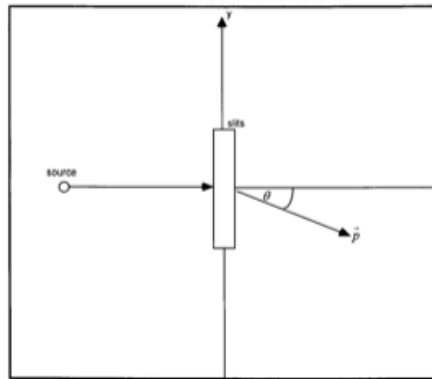
Figure 6.20: Particle Scattering from Slits
