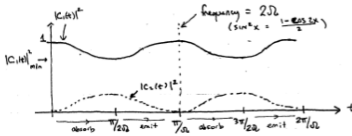
Figure 9.1: Exact Solution
