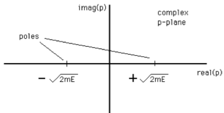
Figure 6.12: Complex p -plane
