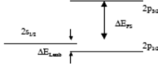
Figure 8.11: n = 2 Spectrum in Hydrogen
