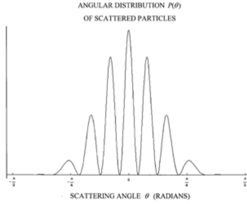
Figure 6.23: Angular Distribution of scattered particles from two slits of finite width The slit width is \lambda = a
