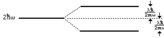
Figure 8.1: Splitting of a degenerate Level
