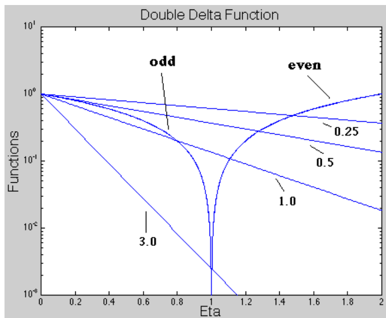
Figure 6.11: Double delta Function Bound States
