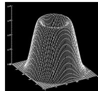
Figure 7.9: |\psi_{11}|^2
