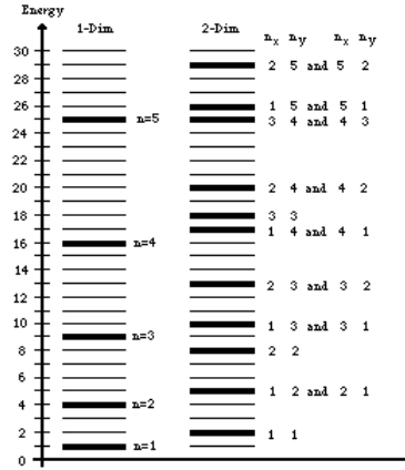
Figure 7.4: Comparison of 1D and 2D Infinite Wells
