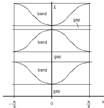
Figure 6.19: Bands and Gaps
