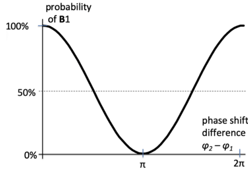
Figure 10.10: Single photon interference, pointing to Dirac's conclusion that "each photon interferes with itself", i.e., each photon follows both paths.
