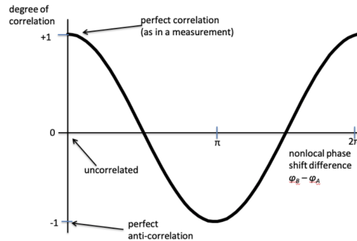
Figure 10.12: The RT0 experiments, demonstrating nonlocality (violation of Bell's inequality). The two photons interfere with each other across an arbitrary distance, i.e., each biphoton interferes with itself.
