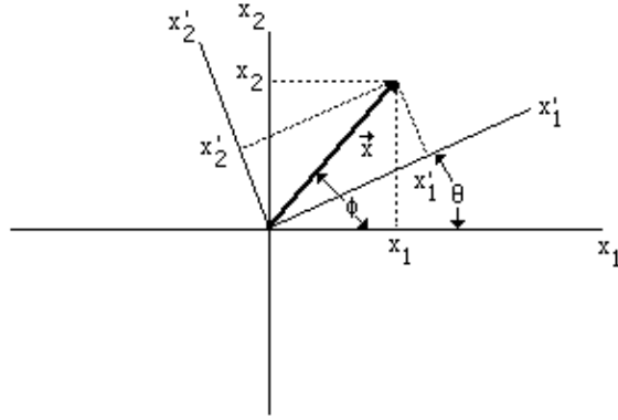
Figure 4.3: Rotation about z-axis
