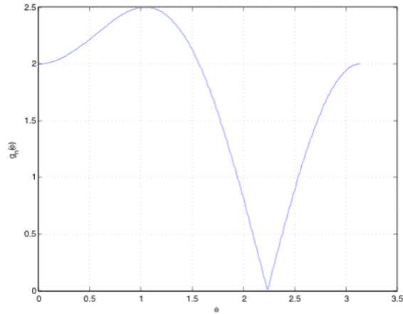
Figure 4.7: Quantum Mechanics versus the Bell Inequality
