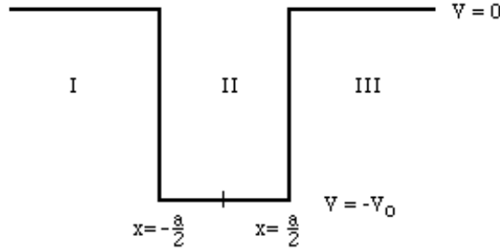
Figure 6.10: Finite Square Well
