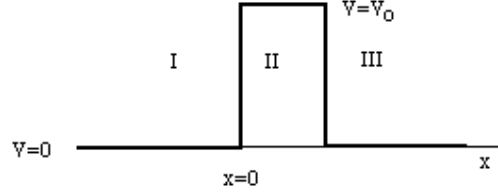
Figure 6.5: Finite Step - Finite Width barrier
