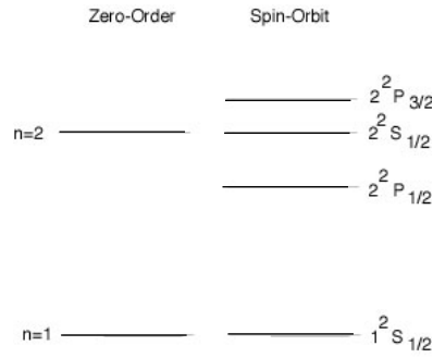
Figure 8.4: Spin-Orbit Energy Levels
