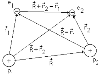
Figure 8.6: Van der Waal's System
