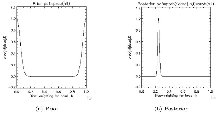
Figure 3.3: Knowledge that it is Unfair
