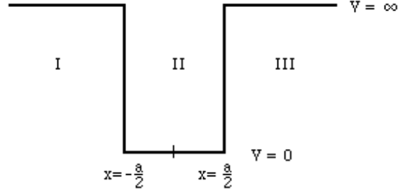
Figure 6.6: Infinite Square Well
