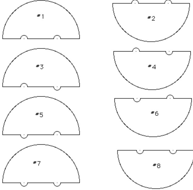
Figure 6.13: Possible Contours
