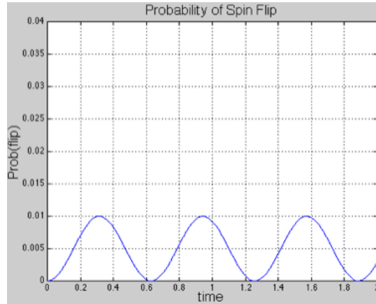
Figure 7.2: Spin=Flip Probability versus Time
