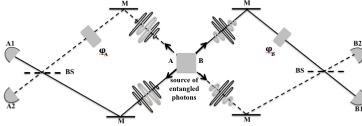
Figure 10.11: The RT0 experiments. In each trial, each of two entangled photons travels two phase-shifted paths (one solid, the other dashed) to beam splitters and coincidence detectors. Think of one biphoton spreading from the source along both the solid and dashed paths.
