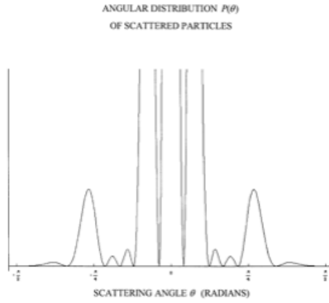
Figure 6.24: Angular Distribution of scattered particles from two slits of finite width The slit width is \lambda = a/2
