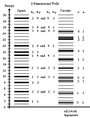
Figure 7.7: Two Dimensional Wells
