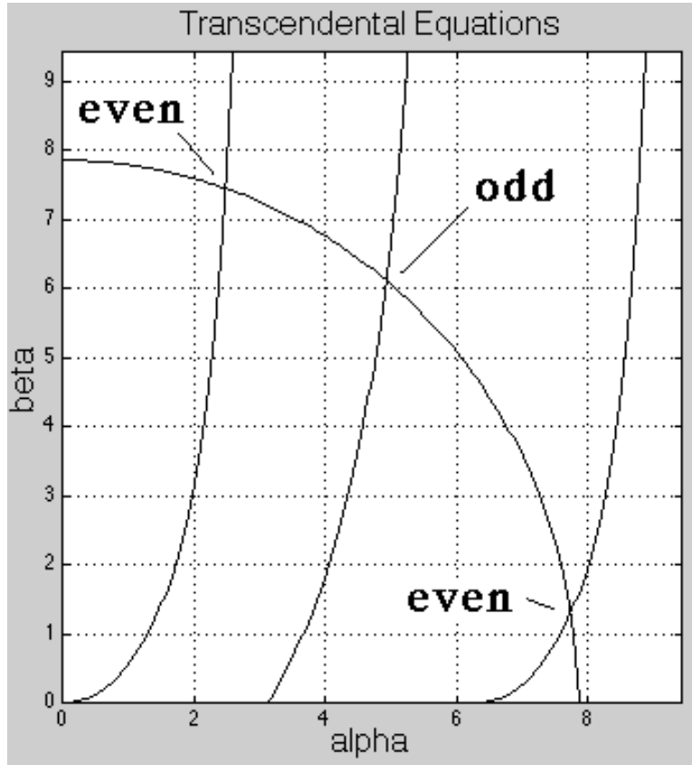
Figure 6.8: Solutions for \sqrt{\frac{2mV_0a^2}{\hbar^2}} = \frac{5\pi}{2}
