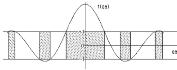
Figure 6.18: Allowed q values
