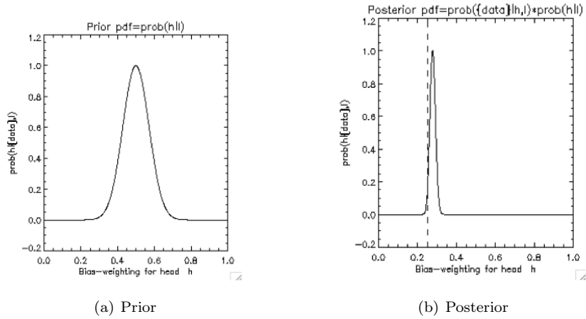
Figure 3.2: Knowledge that Mean is 0.5
