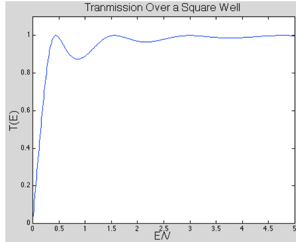
Figure 6.9: Transmission over a Square Well
