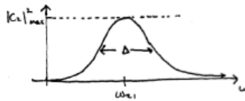
Figure 9.3: Amplitude versus \omega
