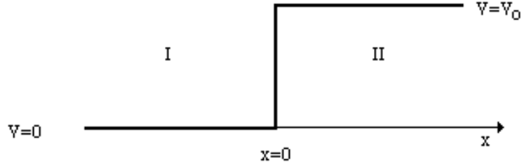
Figure 6.4: Finite Step barrier
