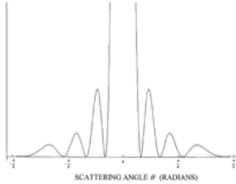
Figure 6.22: Angular Distribution of scattered particles from single slit of finite width
